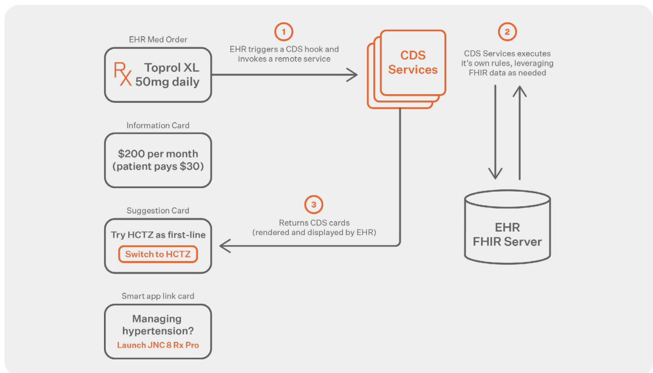
FIGURE 3: Example of CDS-hooks in Operation
