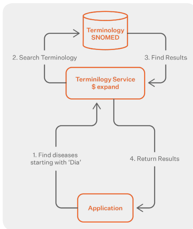
FIGURE 2: Example Terminology Service
