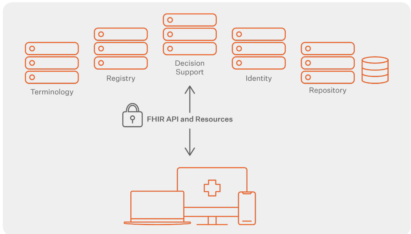
FIGURE 1: FHIR API and Resources
